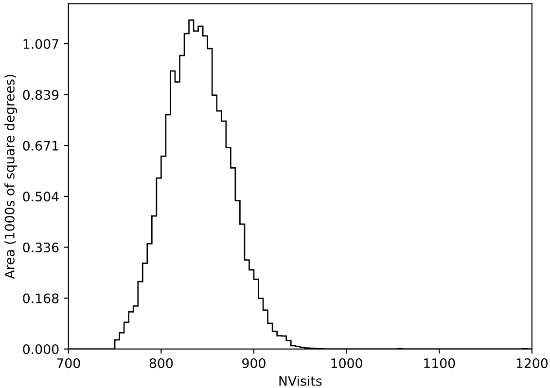
too_elab_r16_d2_griz_v3.4_10yrs WFD all bands: NVisits
