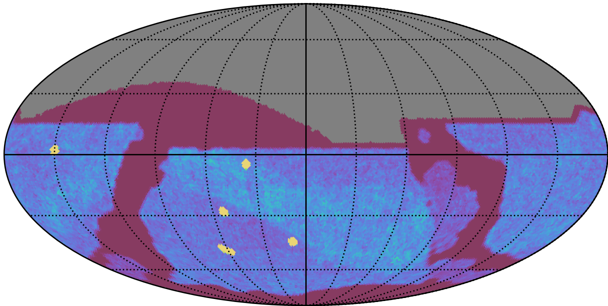
too_elab_r16_d2_griz_v3.4_10yrs All sky z band: NVisits
