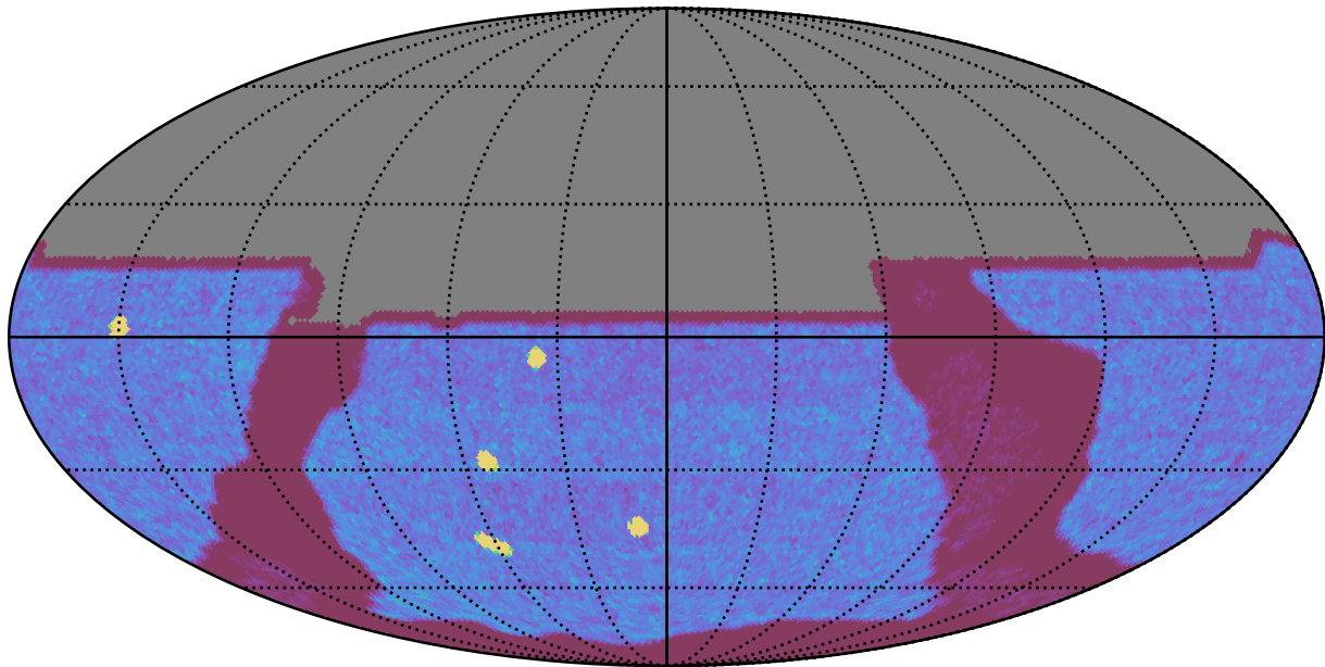
too_elab_r16_d2_griz_v3.4_10yrs All sky y band: NVisits
