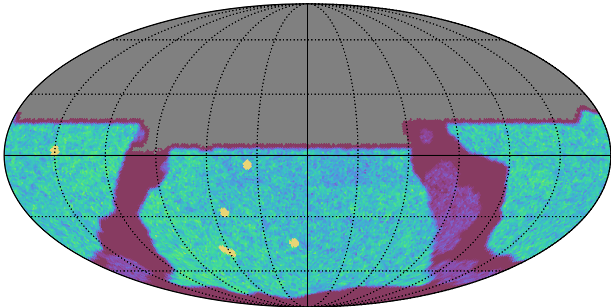
too_elab_r16_d2_griz_v3.4_10yrs All sky u band: NVisits
