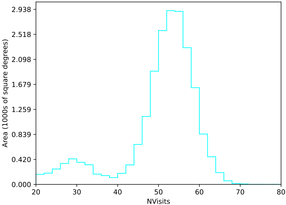
too_elab_r16_d2_griz_v3.4_10yrs All sky u band: NVisits
