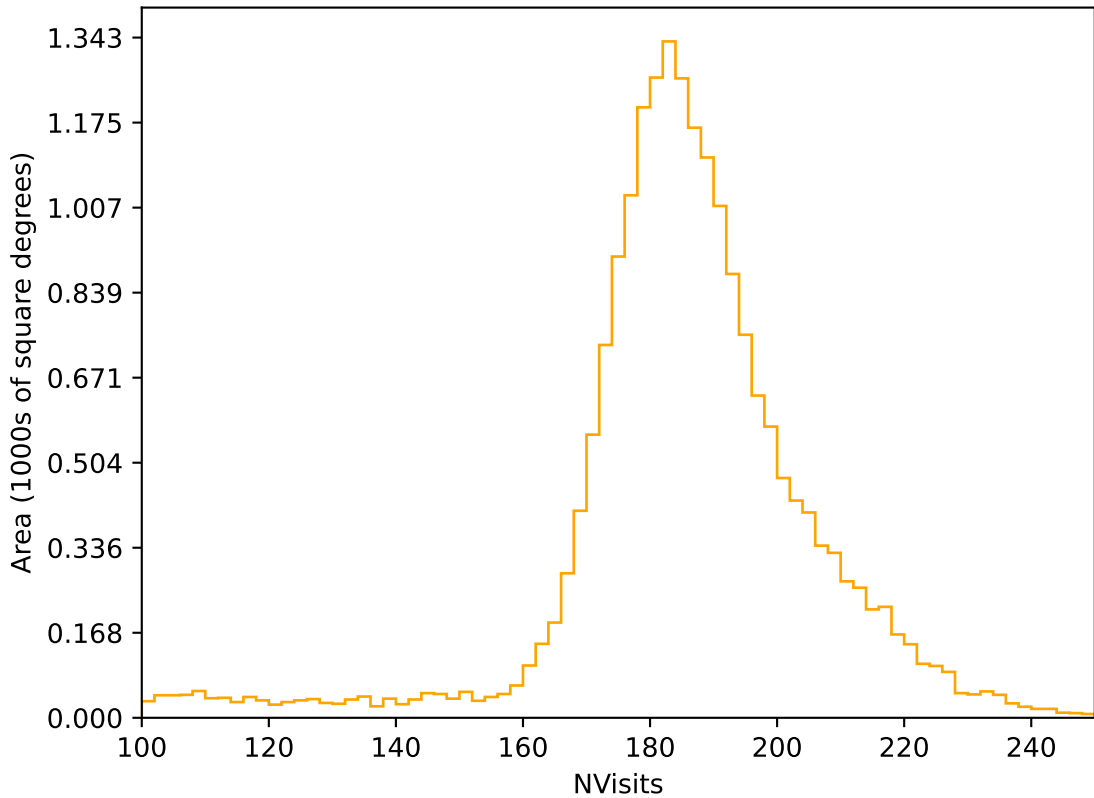
too_elab_r16_d2_griz_v3.4_10yrs All sky r band: NVisits
