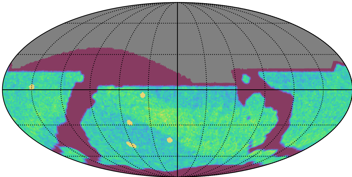
too_elab_r16_d2_griz_v3.4_10yrs All sky i band: NVisits
