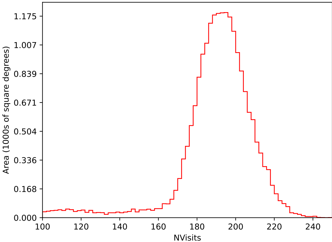
too_elab_r16_d2_griz_v3.4_10yrs All sky i band: NVisits
