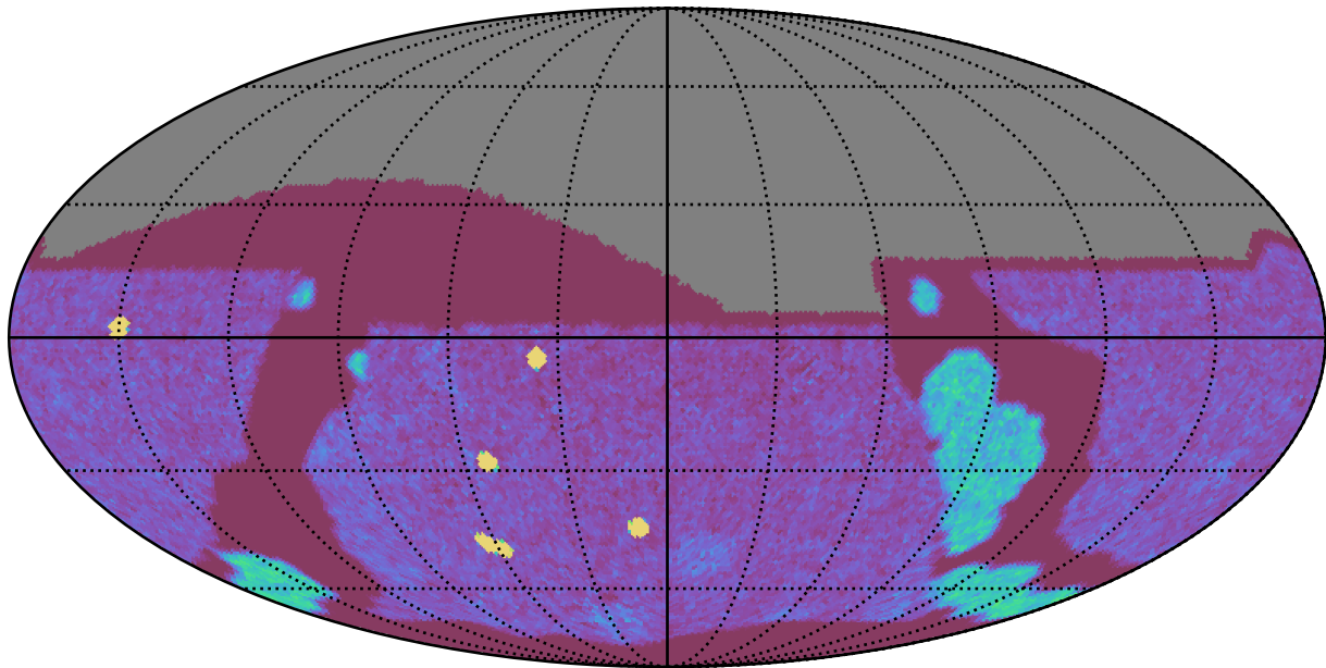
too_elab_r16_d2_griz_v3.4_10yrs All sky g band: NVisits
