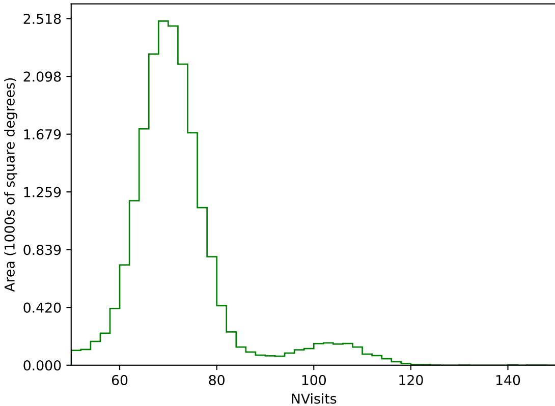
too_elab_r16_d2_griz_v3.4_10yrs All sky g band: NVisits
