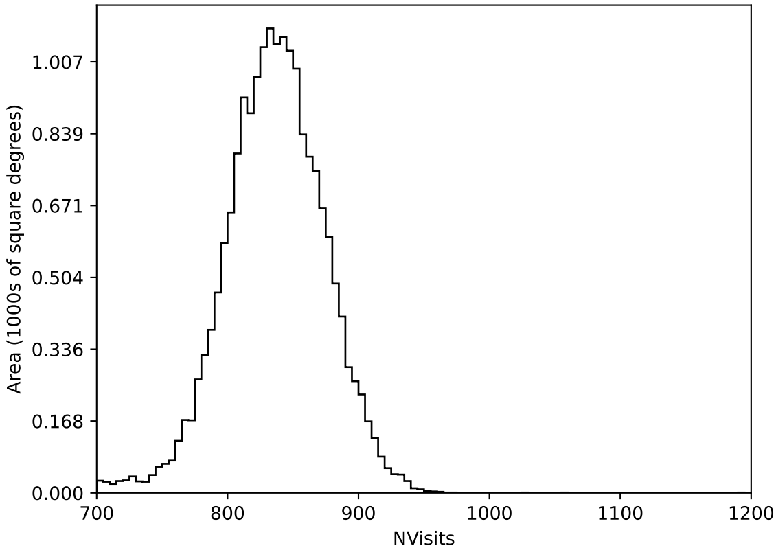
too_elab_r16_d2_griz_v3.4_10yrs All sky all bands: NVisits
