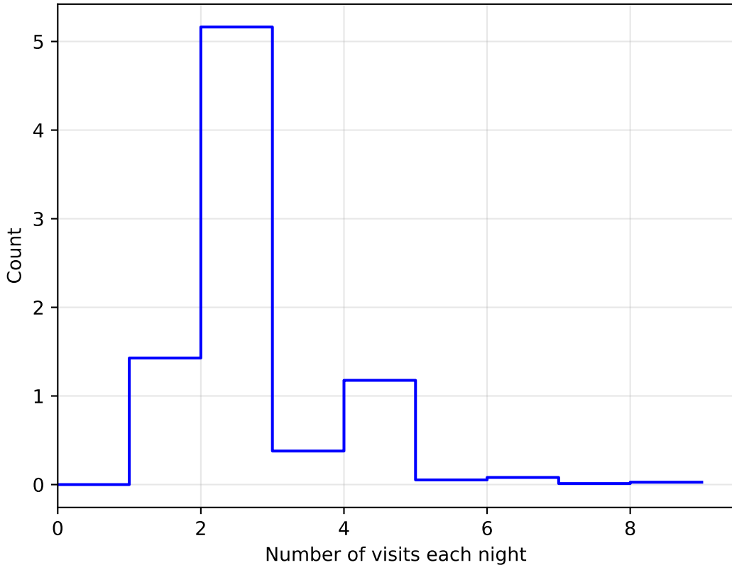
too_elab_r16_d2_griz_v3.4_10yrs WFD: NVisitsPerNight
