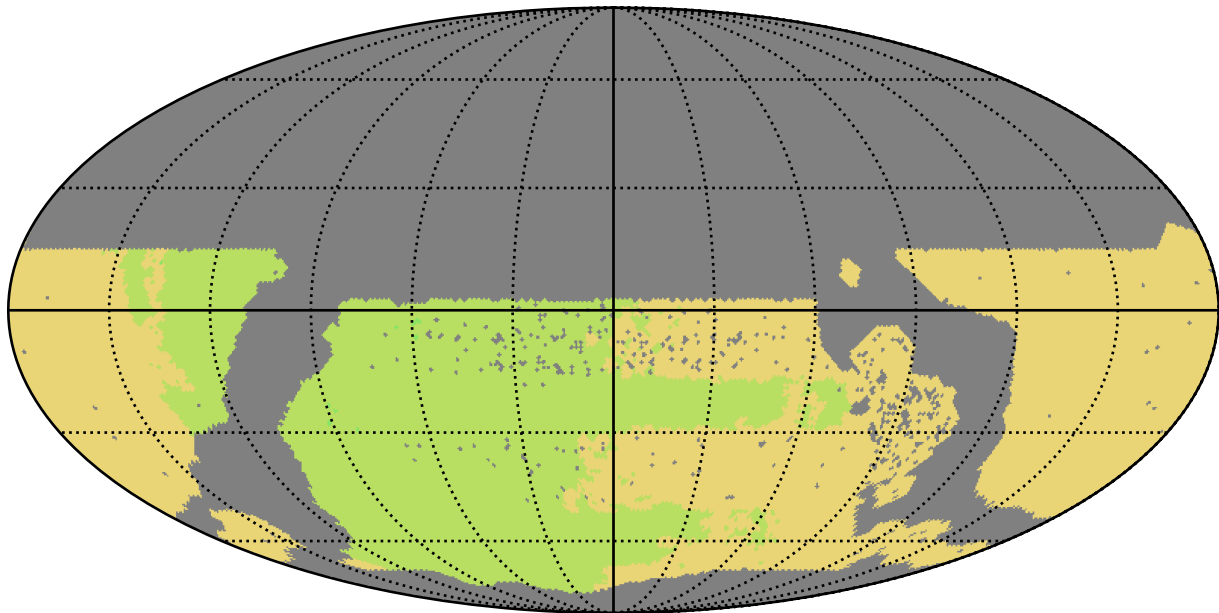
too_elab_r16_d2_griz_v3.4_10yrs WFD all bands: NSeasons
