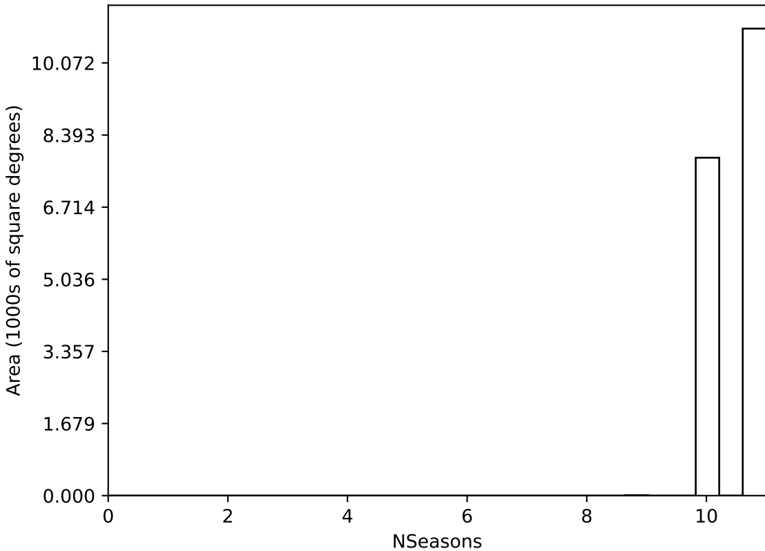
too_elab_r16_d2_griz_v3.4_10yrs WFD all bands: NSeasons
