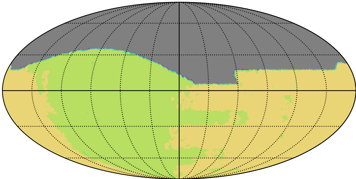
too_elab_r16_d2_griz_v3.4_10yrs All sky all bands: NSeasons
