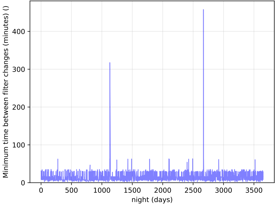
too_elab_r16_d2_griz_v3.4_10yrs Per Night: Minimum time between filter changes (minutes)
