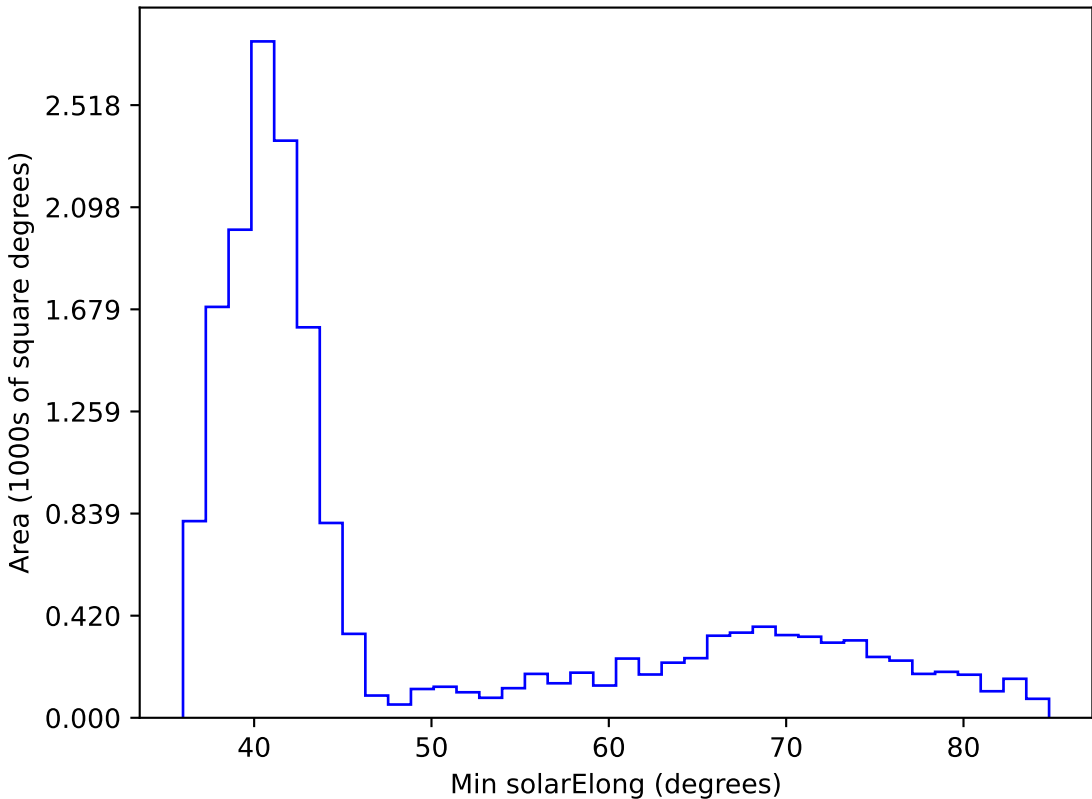
too_elab_r16_d2_griz_v3.4_10yrs WFD z band: Min solarElong
