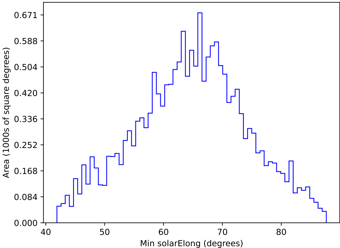
too_elab_r16_d2_griz_v3.4_10yrs WFD y band: Min solarElong
