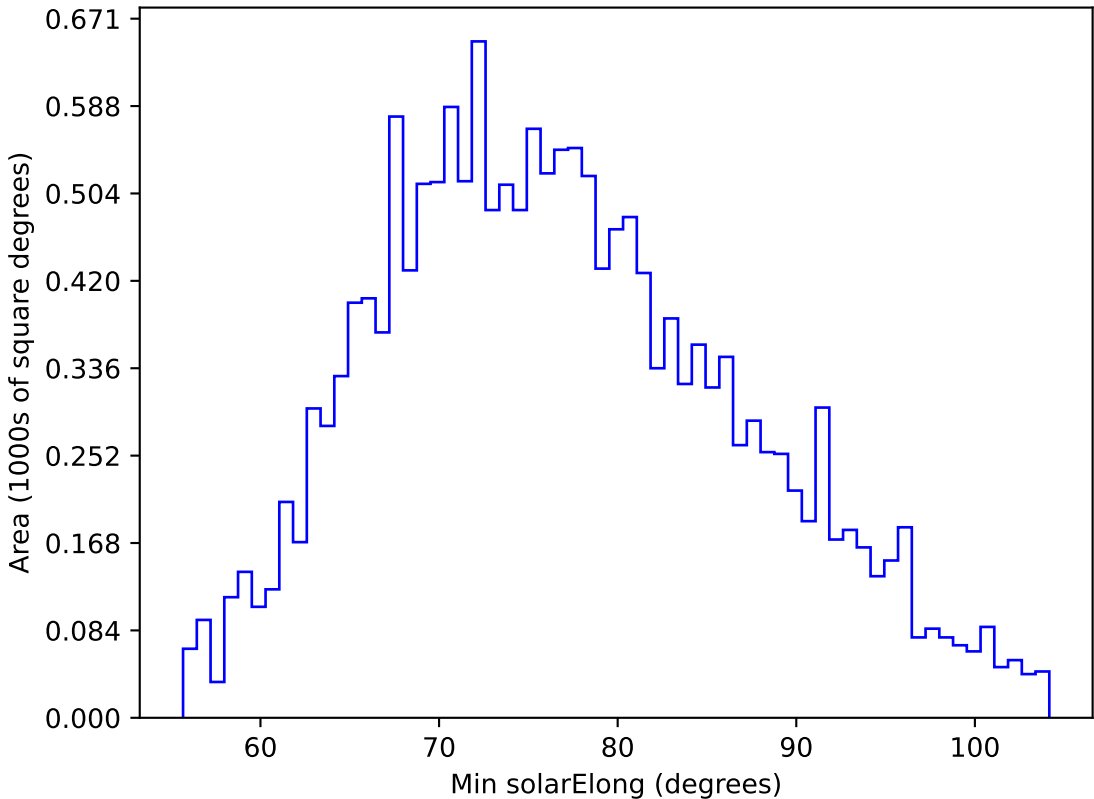
too_elab_r16_d2_griz_v3.4_10yrs WFD u band: Min solarElong
