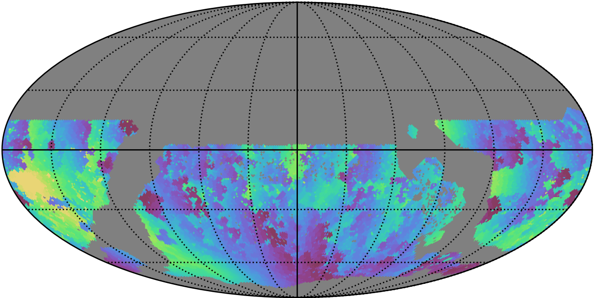
too_elab_r16_d2_griz_v3.4_10yrs WFD g band: Min solarElong
