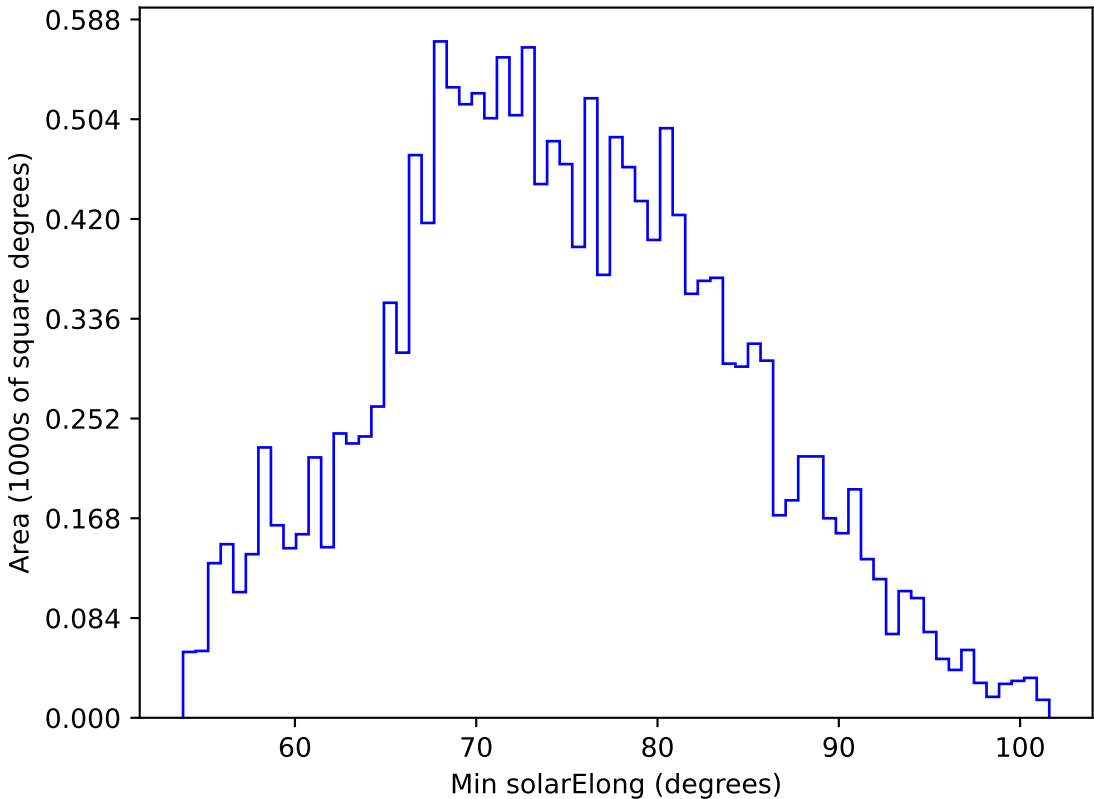
too_elab_r16_d2_griz_v3.4_10yrs WFD g band: Min solarElong
