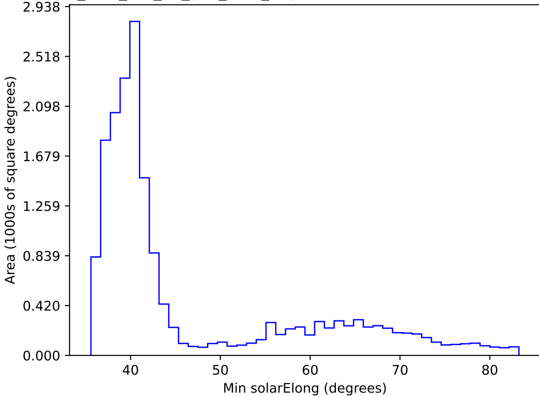
too_elab_r16_d2_griz_v3.4_10yrs WFD all bands: Min solarElong
