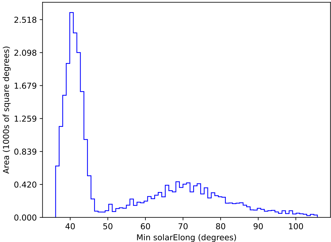
too_elab_r16_d2_griz_v3.4_10yrs All sky z band: Min solarElong
