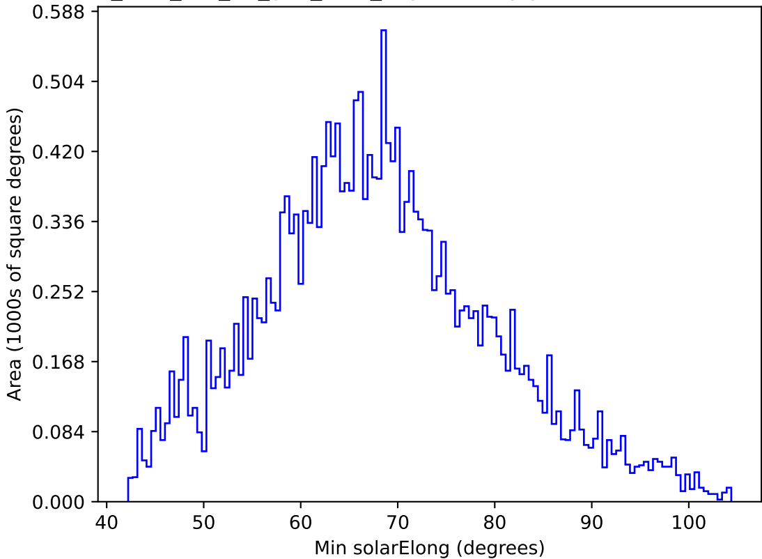
too_elab_r16_d2_griz_v3.4_10yrs All sky y band: Min solarElong
