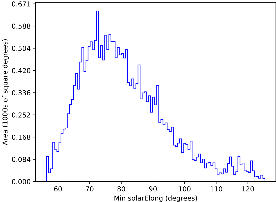
too_elab_r16_d2_griz_v3.4_10yrs All sky u band: Min solarElong
