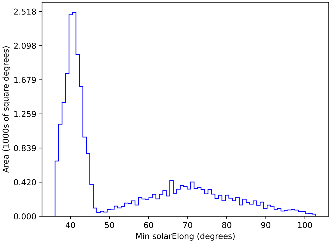
too_elab_r16_d2_griz_v3.4_10yrs All sky i band: Min solarElong
