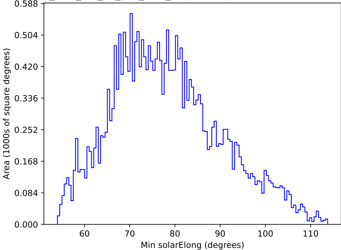
too_elab_r16_d2_griz_v3.4_10yrs All sky g band: Min solarElong
