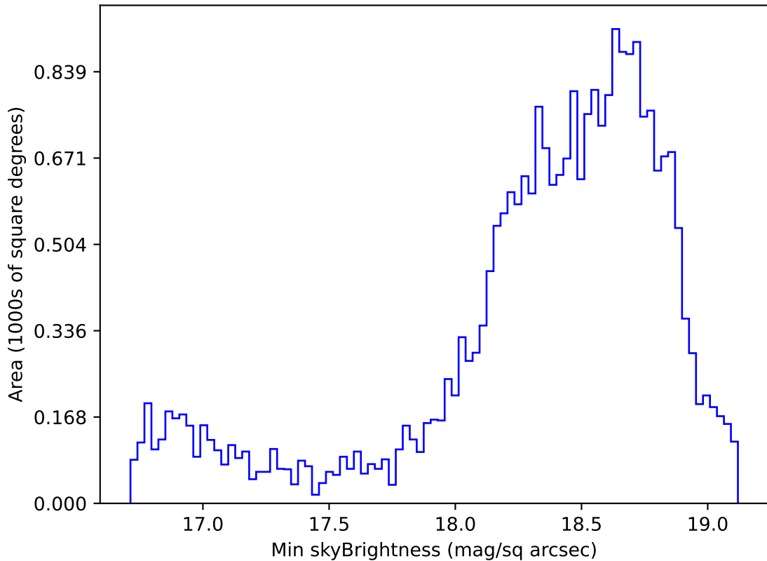
too_elab_r16_d2_griz_v3.4_10yrs Yr 1 z band: Min skyBrightness
