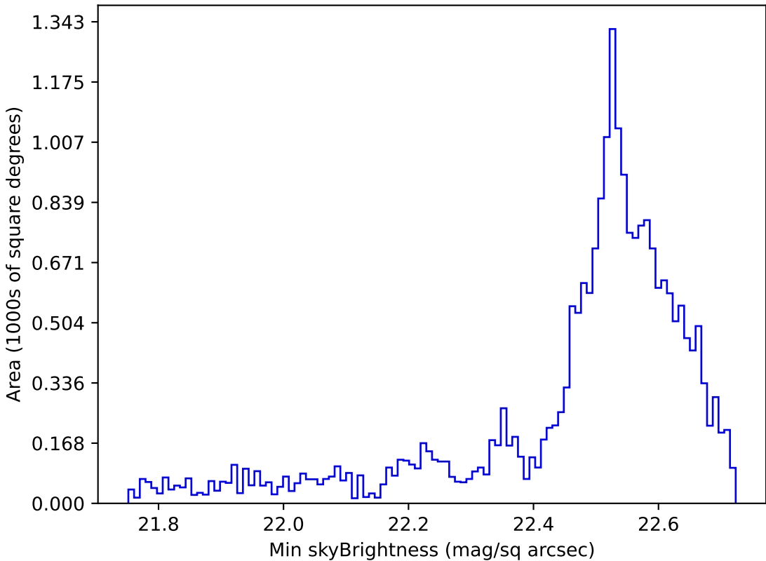
too_elab_r16_d2_griz_v3.4_10yrs Yr 1 u band: Min skyBrightness
