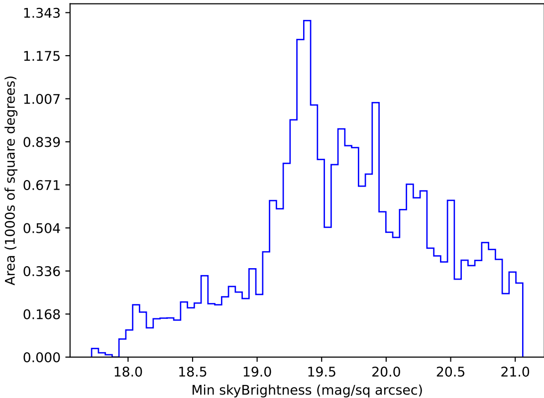
too_elab_r16_d2_griz_v3.4_10yrs Yr 1 r band: Min skyBrightness
