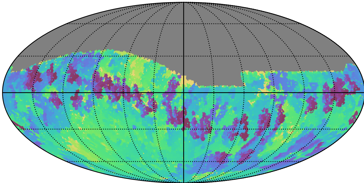
too_elab_r16_d2_griz_v3.4_10yrs Yr 1 i band: Min skyBrightness
