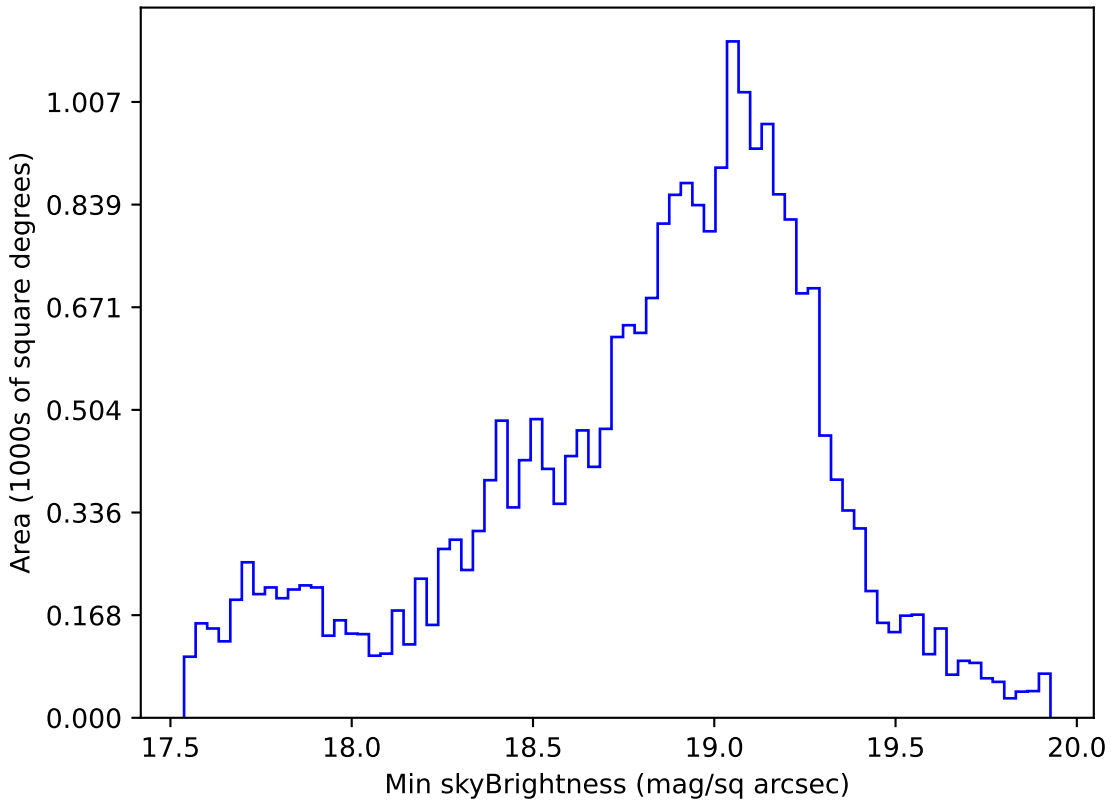
too_elab_r16_d2_griz_v3.4_10yrs Yr 1 i band: Min skyBrightness
