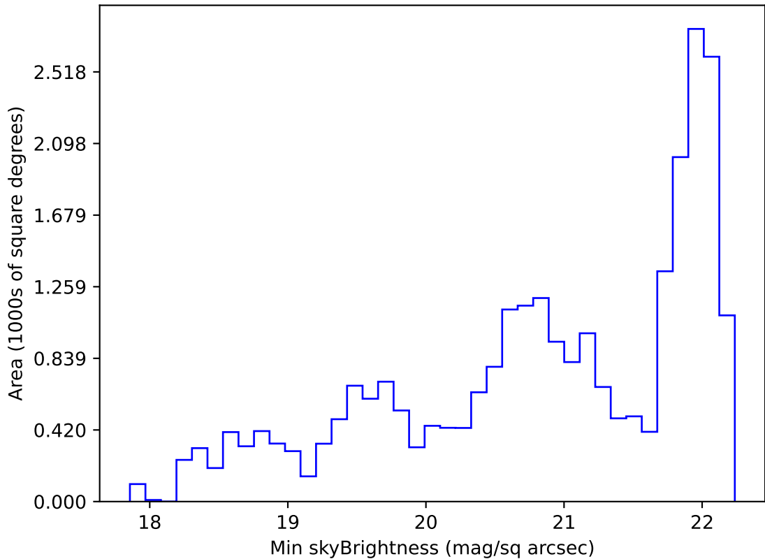
too_elab_r16_d2_griz_v3.4_10yrs Yr 1 g band: Min skyBrightness
