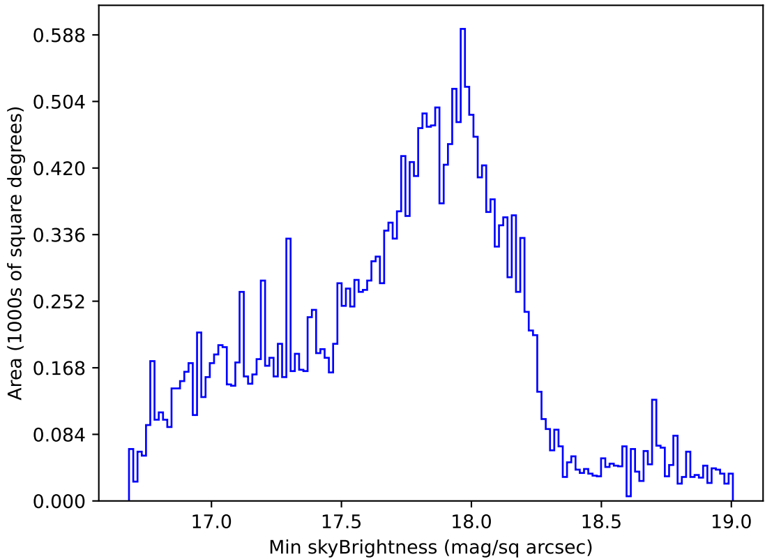
too_elab_r16_d2_griz_v3.4_10yrs Yr 1 all bands: Min skyBrightness
