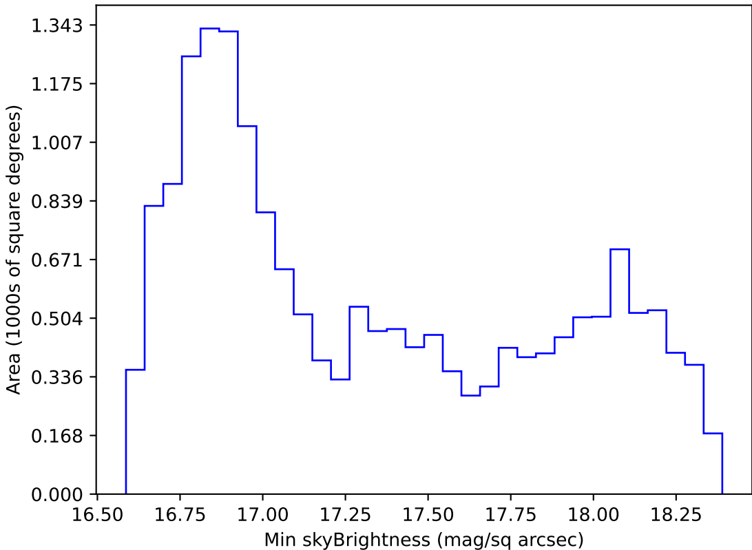
too_elab_r16_d2_griz_v3.4_10yrs WFD z band: Min skyBrightness
