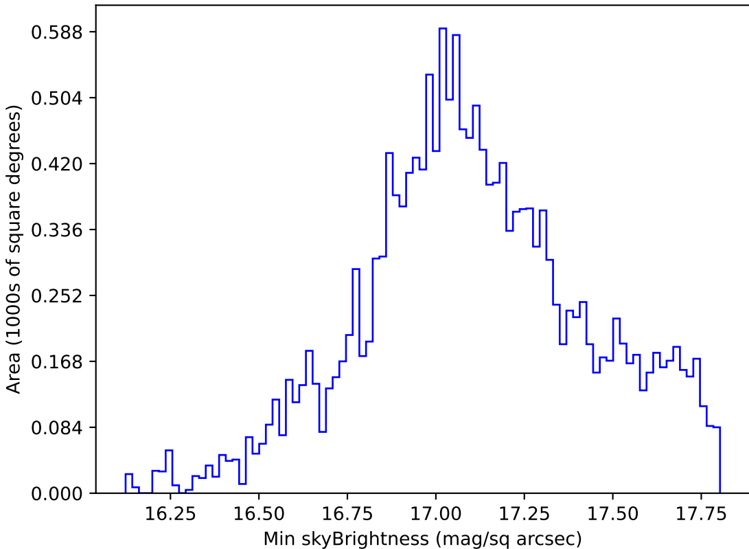
too_elab_r16_d2_griz_v3.4_10yrs WFD y band: Min skyBrightness
