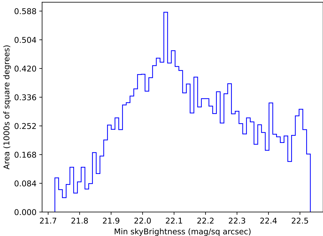
too_elab_r16_d2_griz_v3.4_10yrs WFD u band: Min skyBrightness
