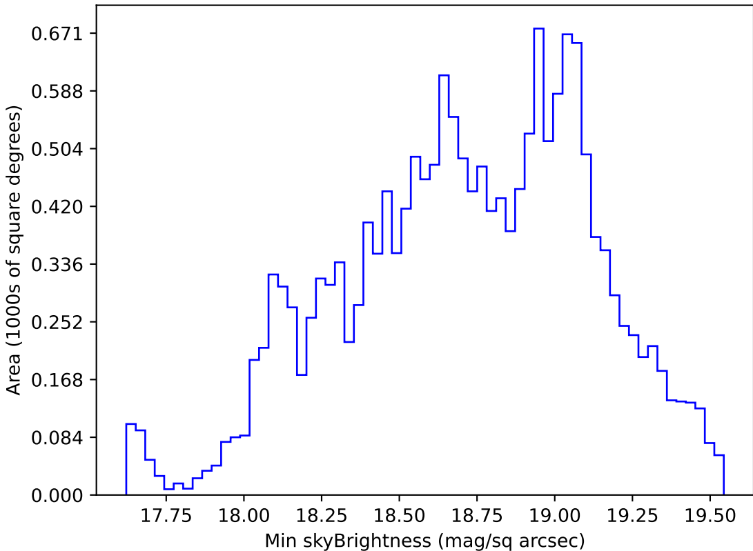
too_elab_r16_d2_griz_v3.4_10yrs WFD r band: Min skyBrightness
