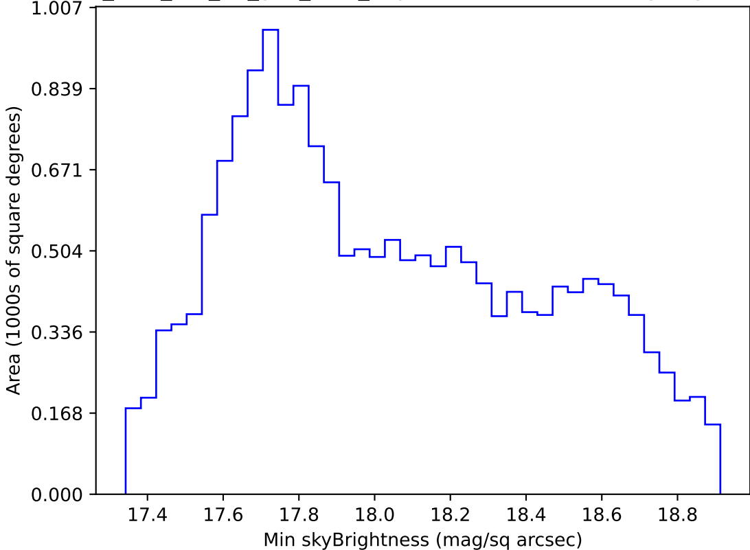
too_elab_r16_d2_griz_v3.4_10yrs WFD i band: Min skyBrightness
