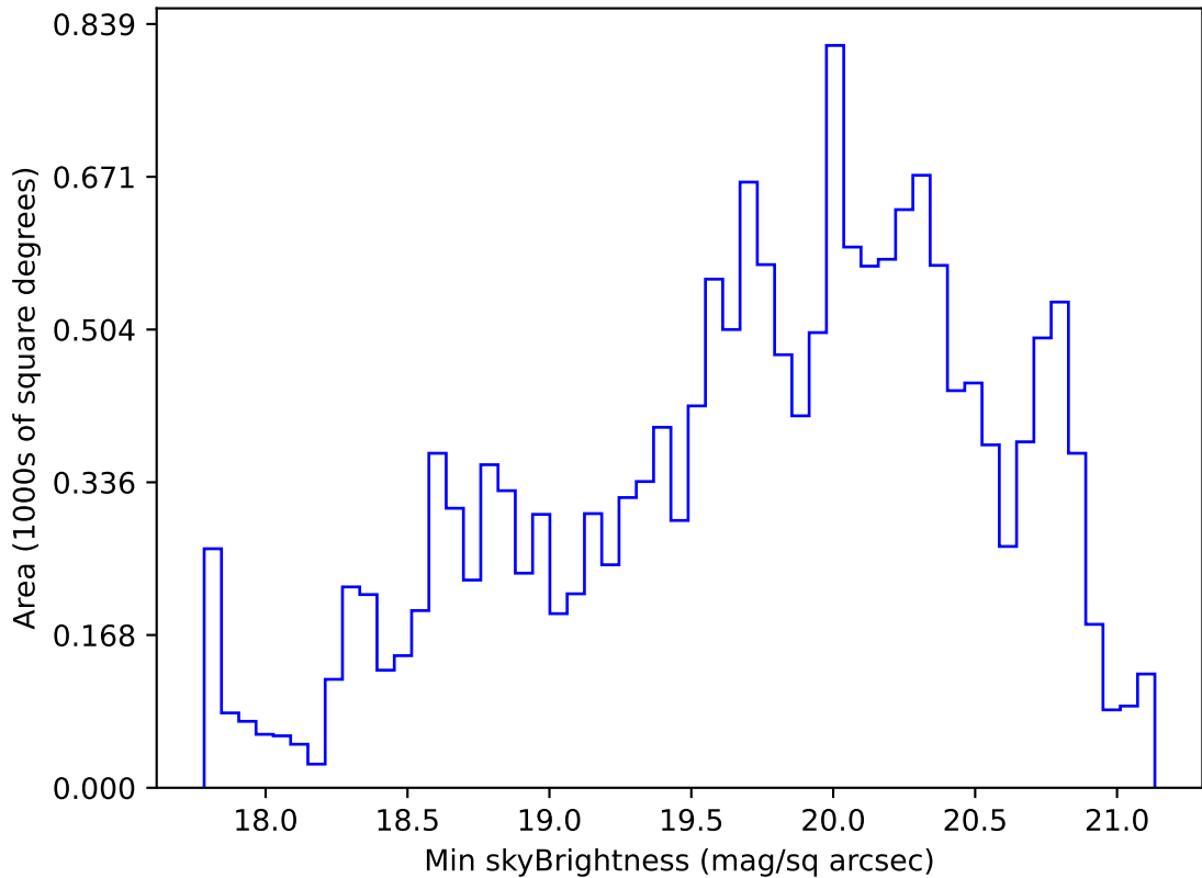
too_elab_r16_d2_griz_v3.4_10yrs WFD g band: Min skyBrightness
