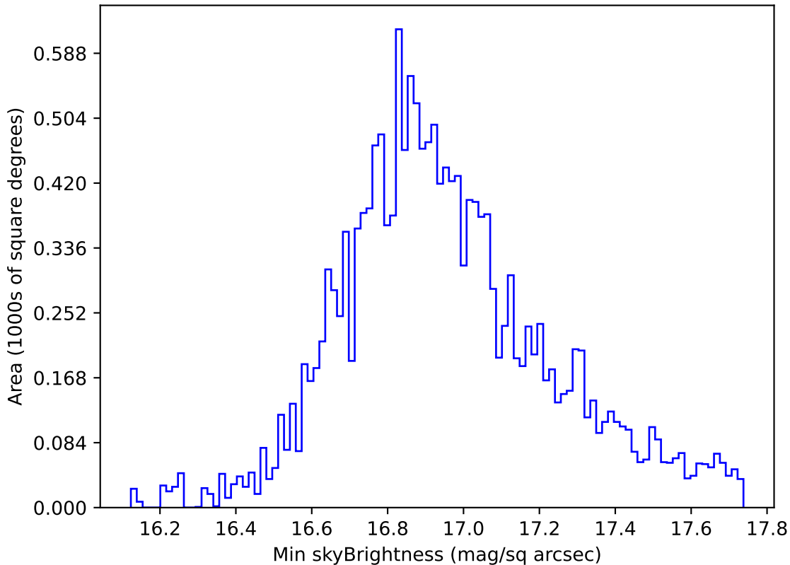
too_elab_r16_d2_griz_v3.4_10yrs WFD all bands: Min skyBrightness
