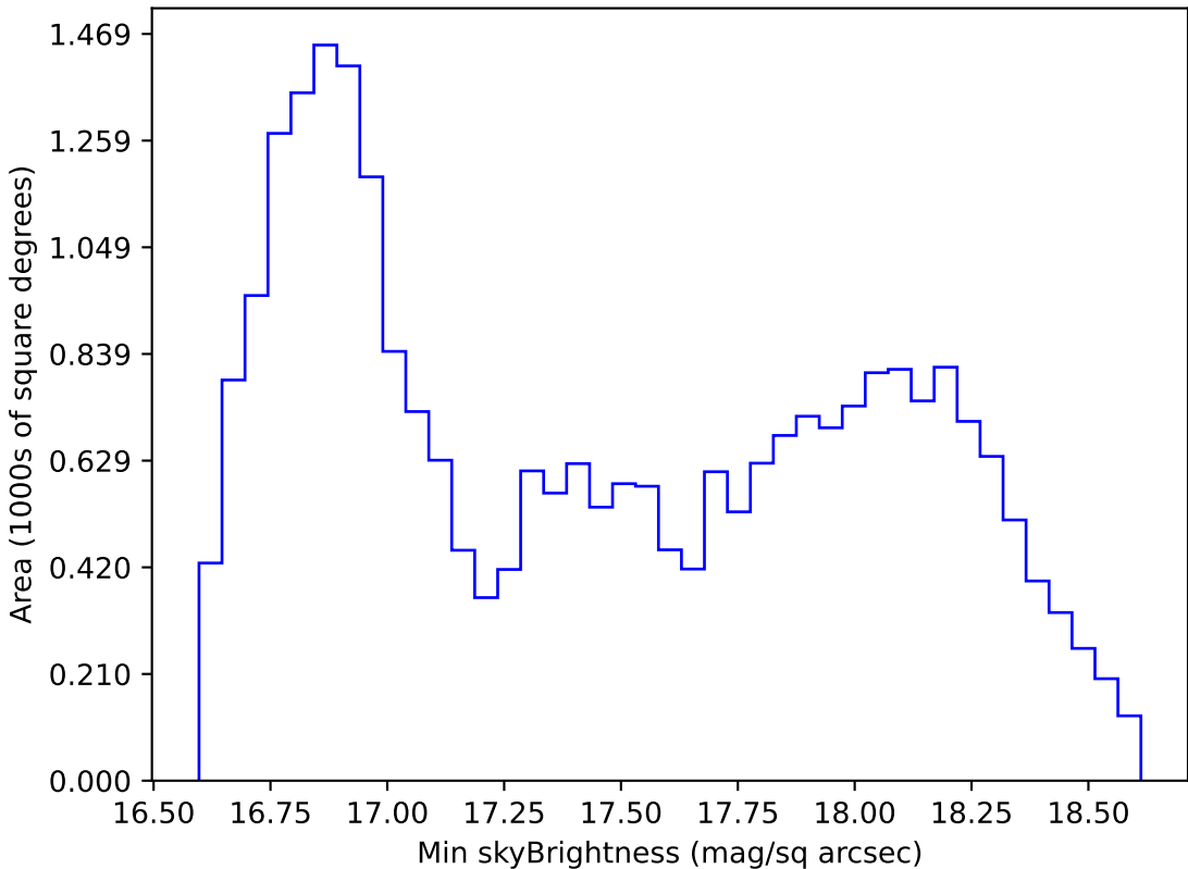
too_elab_r16_d2_griz_v3.4_10yrs All sky z band: Min skyBrightness
