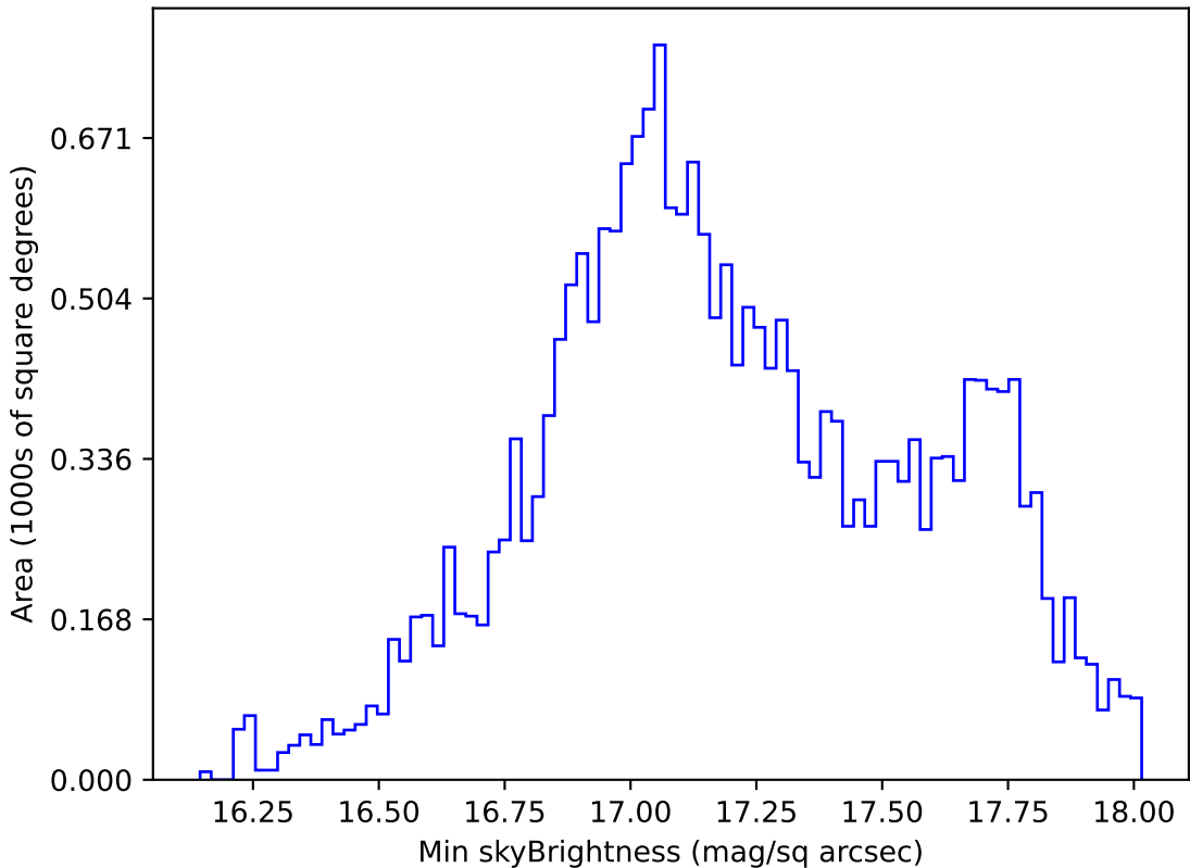
too_elab_r16_d2_griz_v3.4_10yrs All sky y band: Min skyBrightness
