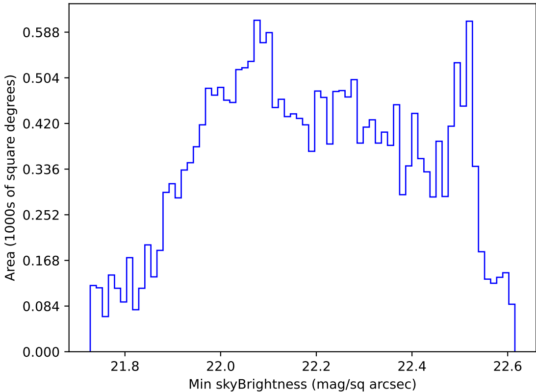
too_elab_r16_d2_griz_v3.4_10yrs All sky u band: Min skyBrightness
