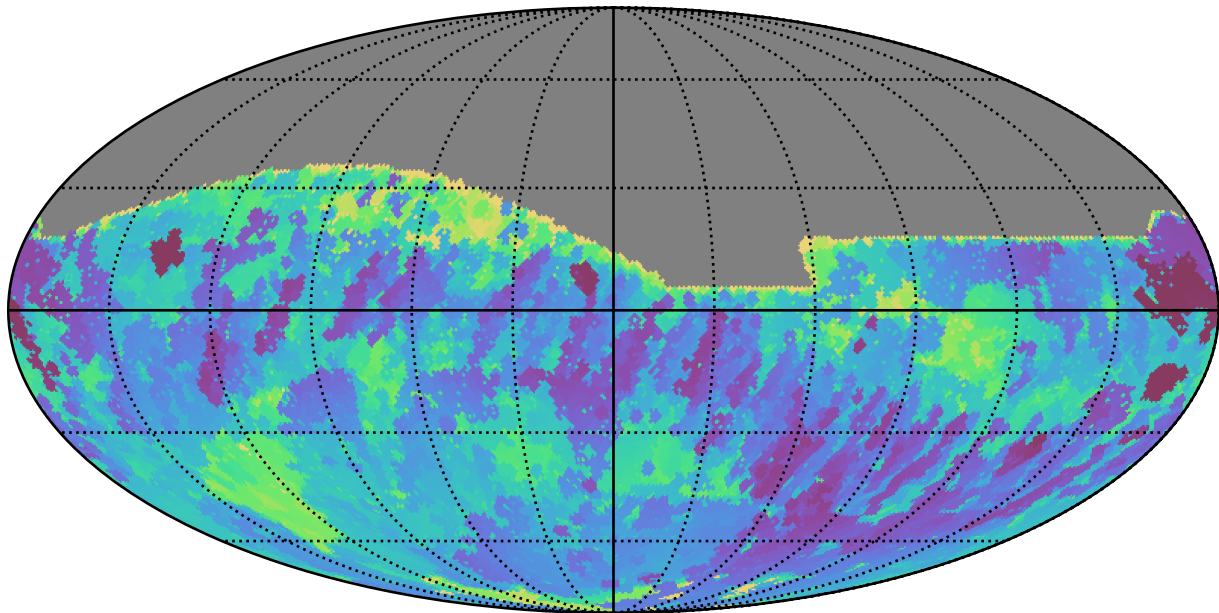
too_elab_r16_d2_griz_v3.4_10yrs All sky r band: Min skyBrightness
