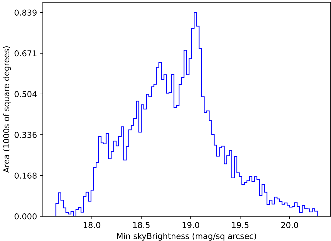
too_elab_r16_d2_griz_v3.4_10yrs All sky r band: Min skyBrightness
