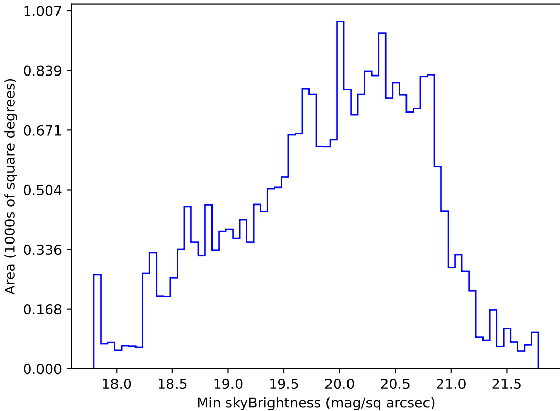
too_elab_r16_d2_griz_v3.4_10yrs All sky g band: Min skyBrightness
