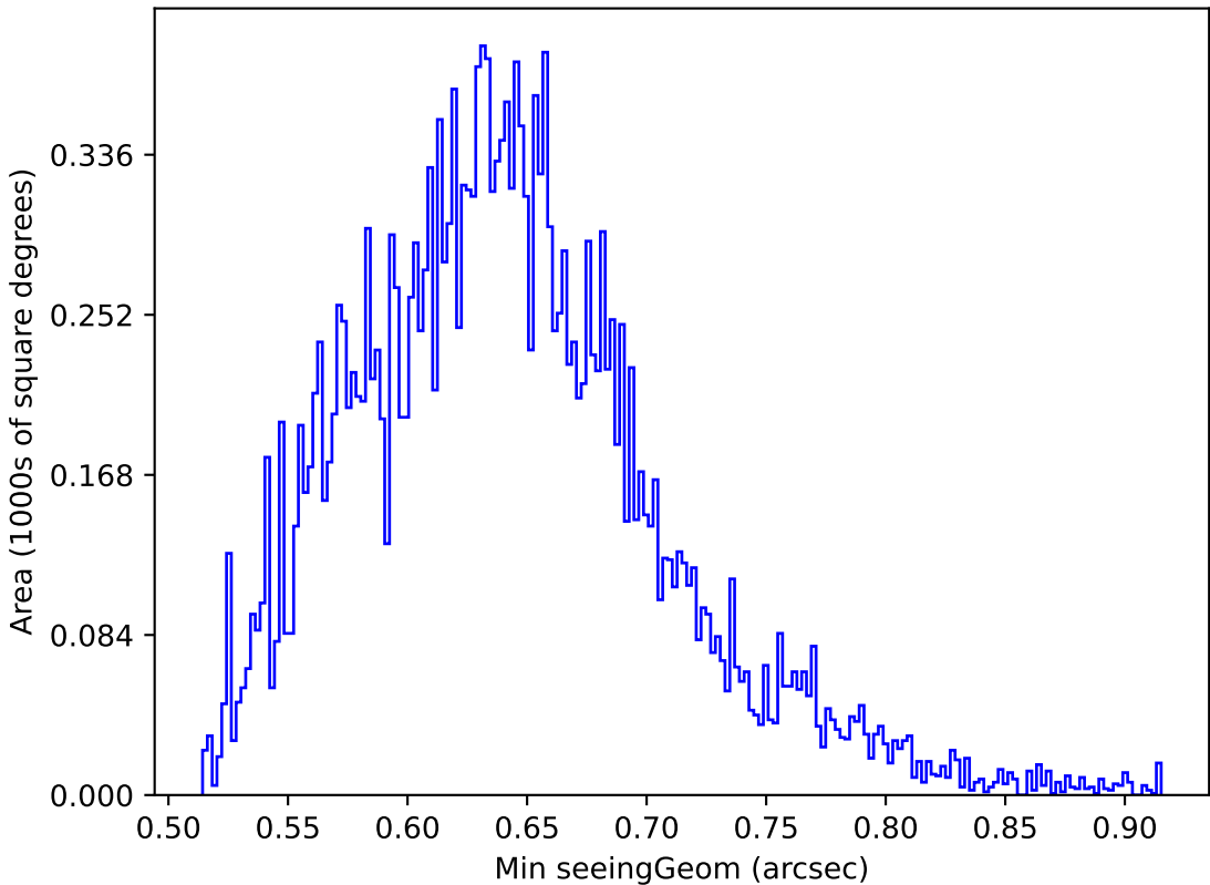
too_elab_r16_d2_griz_v3.4_10yrs Yr 1 y band: Min seeingGeom
