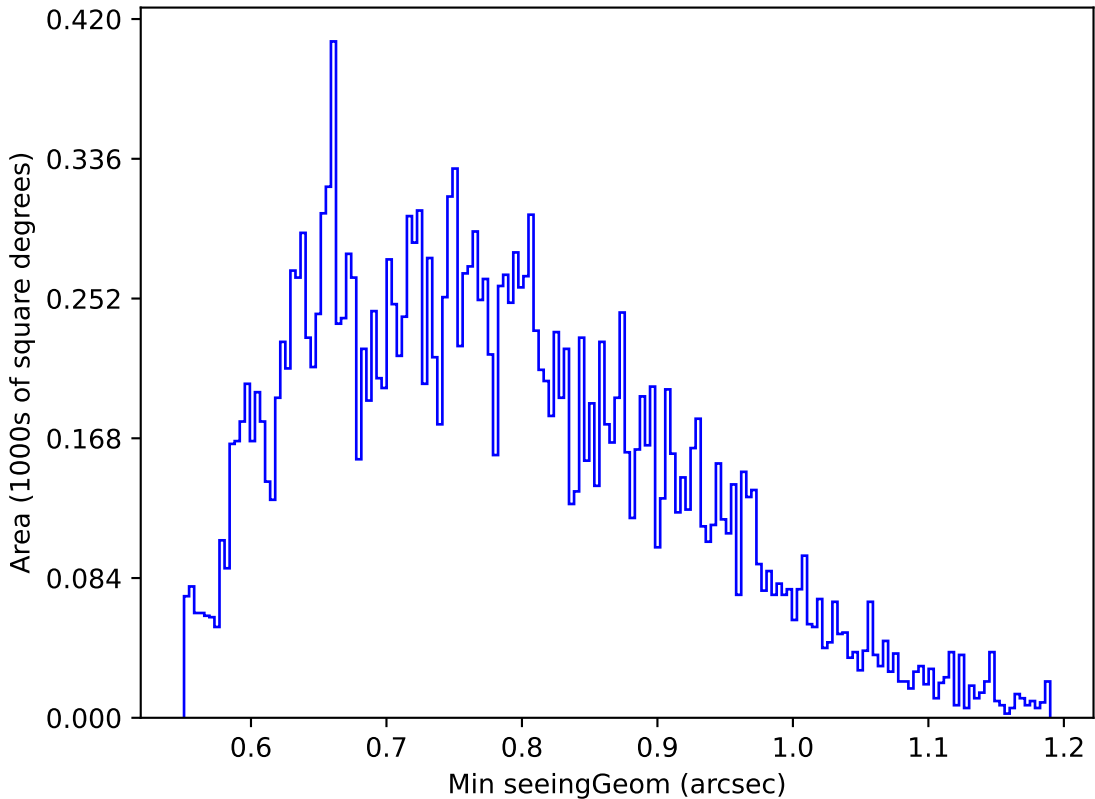
too_elab_r16_d2_griz_v3.4_10yrs Yr 1 u band: Min seeingGeom
