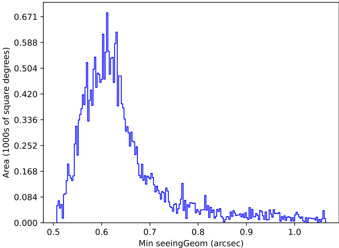
too_elab_r16_d2_griz_v3.4_10yrs Yr 1 r band: Min seeingGeom
